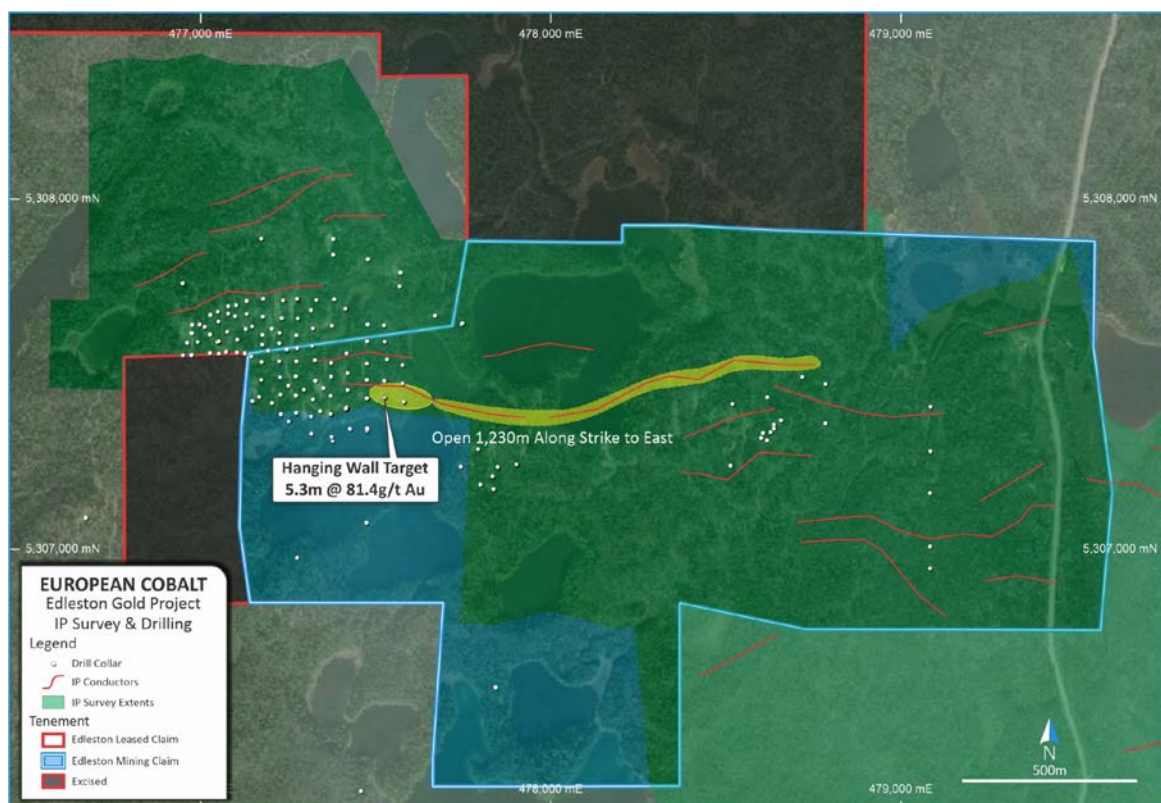
Figure 4: Edleston Hangingwall Target, IP Conductors & Drilling
