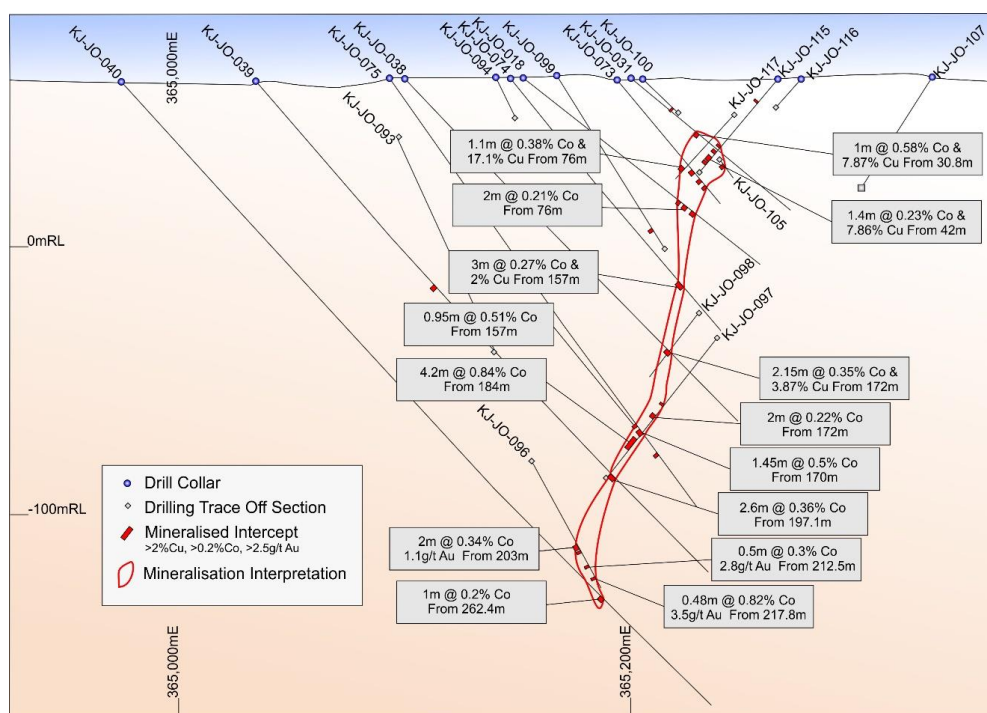
Figure 9: Joughineva Drill Section
