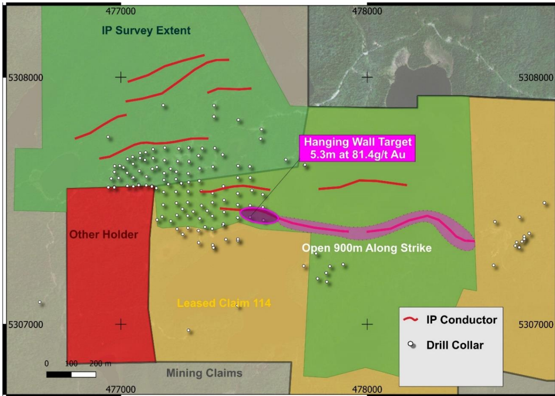
FIGURE 6: IP SURVEY & DRILLING
