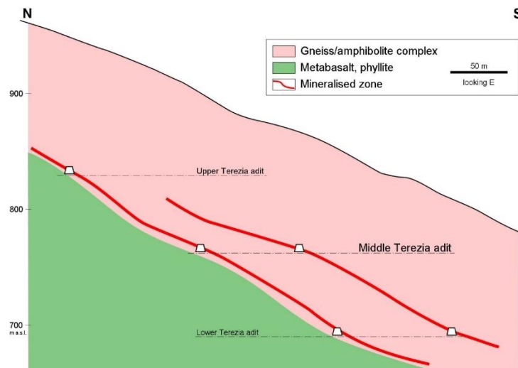
Figure 14: Section View of Middle Terezia Adit
