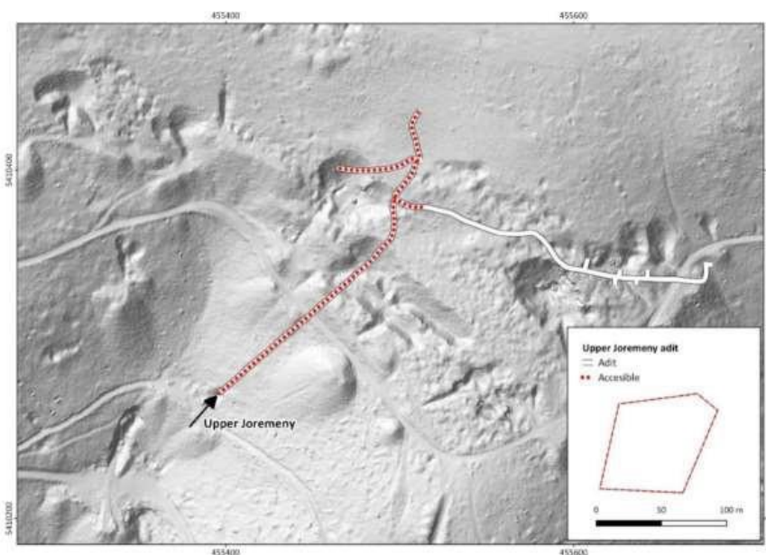
Figure 12: Current underground development and areas accessible in the Upper Joremeny Adit
